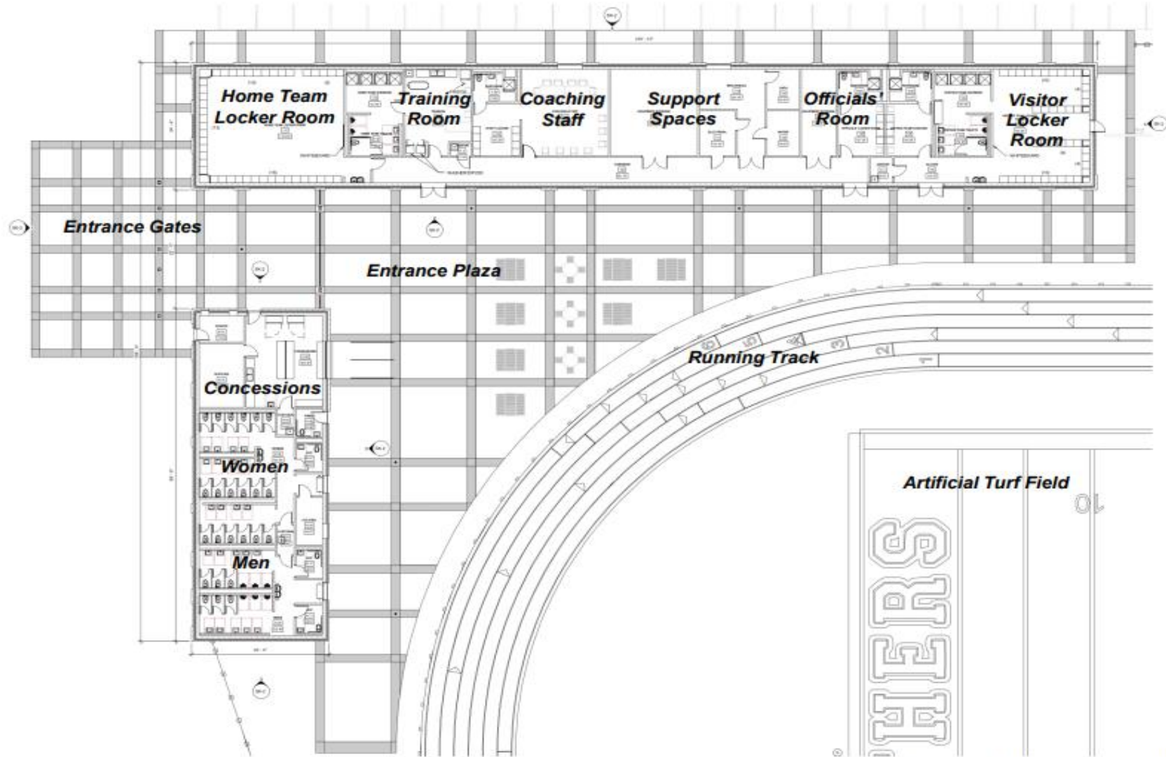
Proposed Fieldhouse + Amenities Building Floor Plans
